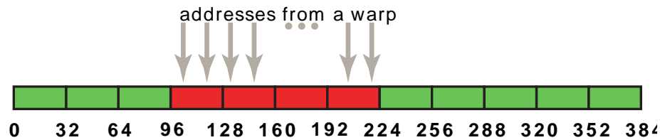
Figure 3 Coalesced access
